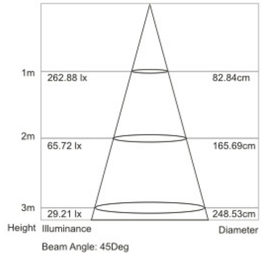
Lux-Distance Curve
